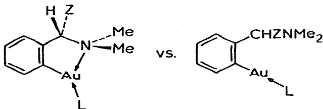
Fig. 1. Possible coordination geometries of Au I in 2-Me 2 NCHZC 6 H 4 AuPPh 3 (I; Z = H and II; Z = Me).
